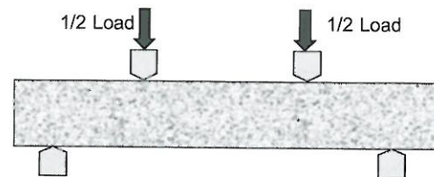
ASTM C 78 - Third-Point Loading - half the load is applied at each third of the span length. MR is lower than center-point loading. Maximum stress is present over the center 1/3 portion of the beam
