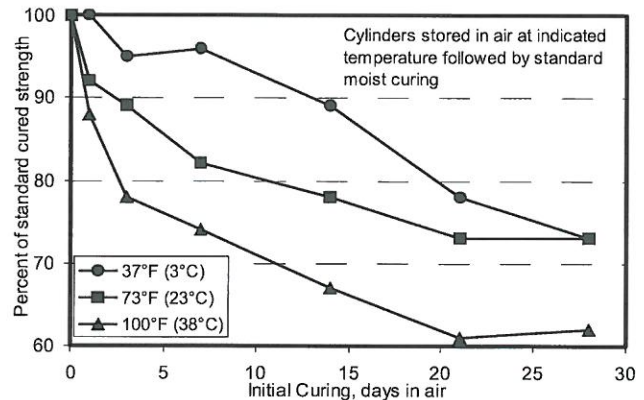
Effect of Non-Standard Curing on Compressive Strength (Ref 5)
